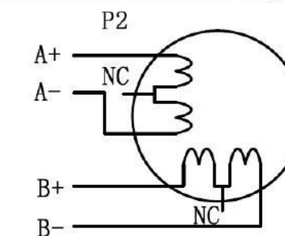
Figure 7: 6-lead motor full coil (higher torque) connections
