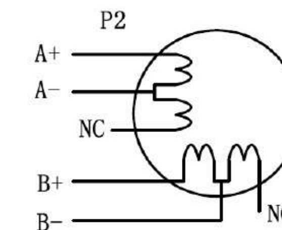
Figure 6: 6-lead motor half coil (higher speed) connections
