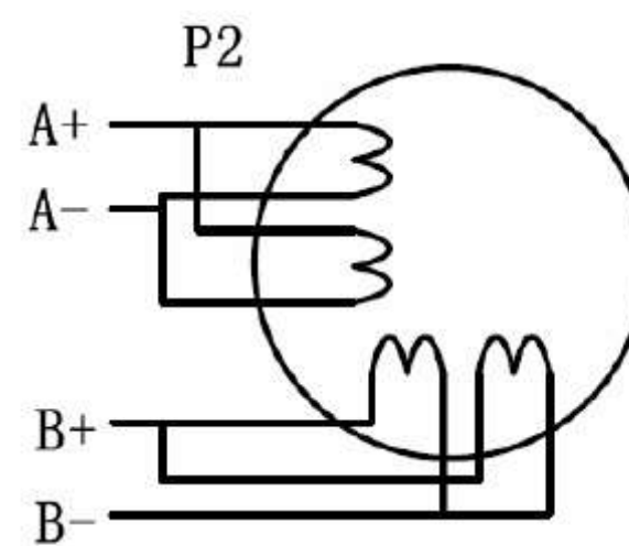
Figure 9: 8-lead motor parallel connections
