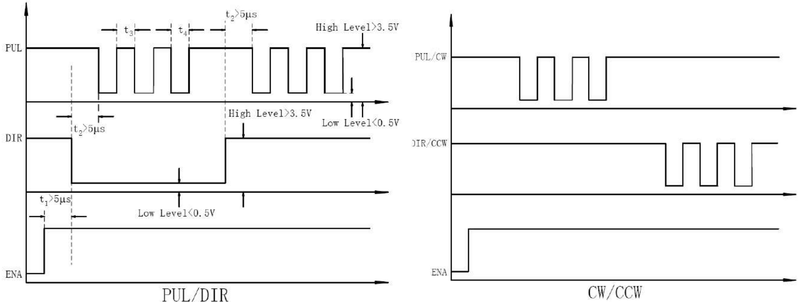
Figure 11: Sequence chart of control signals
