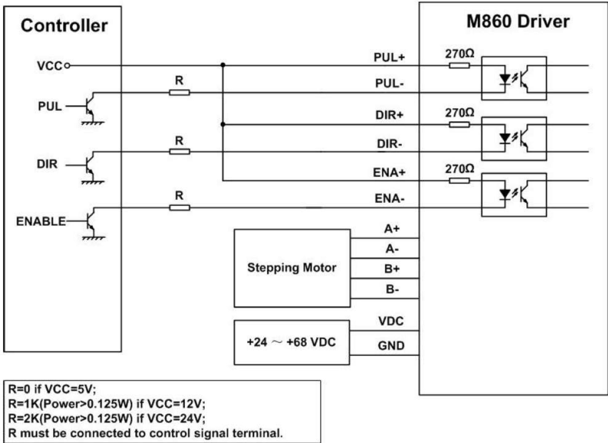
Figure 10: Typical connection
