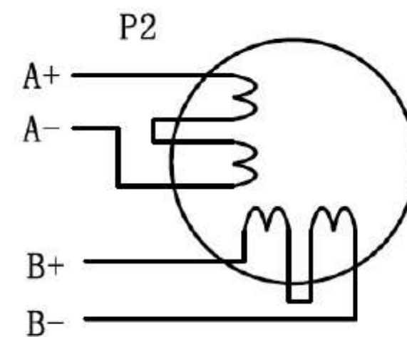
Figure 8: 8-lead motor series connections
