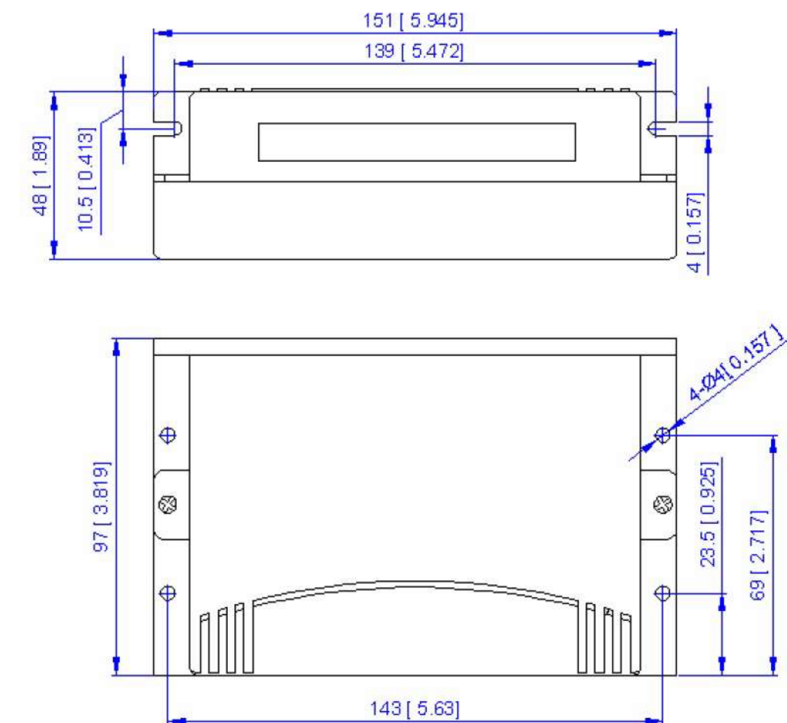
Figure 1: Mechanical specifications
