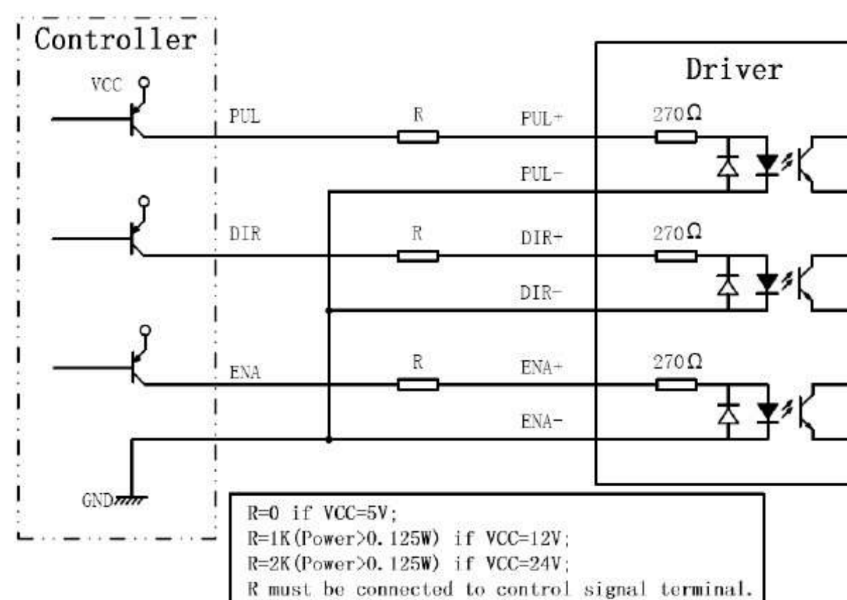
Figure 4: Connection to PNP signal (common-cathode)
