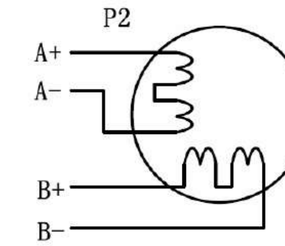
Figure 5: 4-lead Motor Connections
