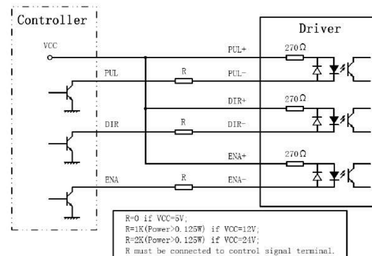
Figure 3: Connections to open-collector signal (common-anode)
